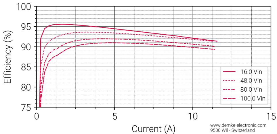
Figure 2 Efficiency in the constant voltage range of the DC-Transformer 145E-13.8-SD
