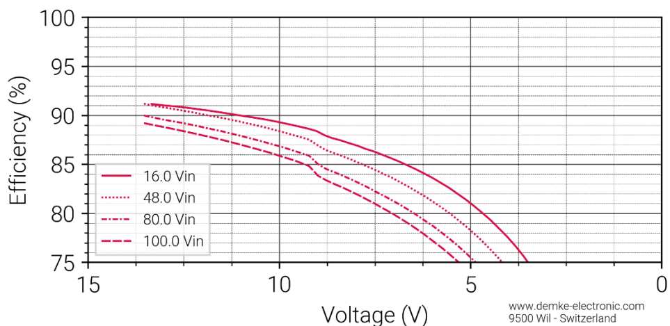
Figure 3 Efficiency in the constant current range of the DC-Transformer 145E-13.8-SD
