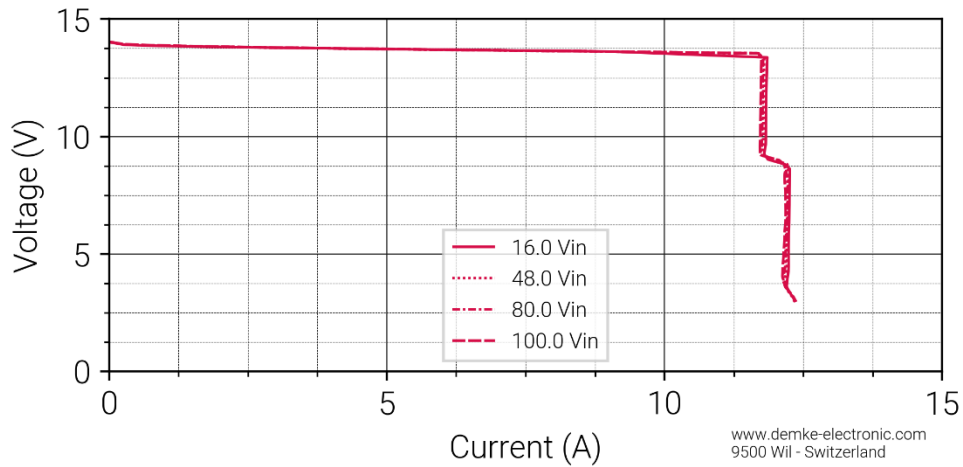
Figure 1 Voltage against current of the DC-Transformer 145E-13.8-SD
