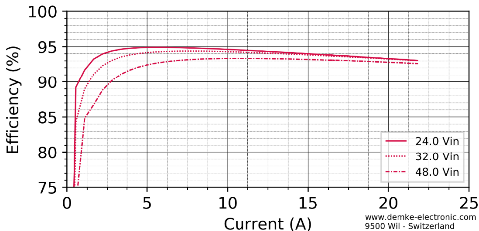
Figure 2 Efficiency in the constant voltage range of the DC-Transformer 151DH-13.8-On
