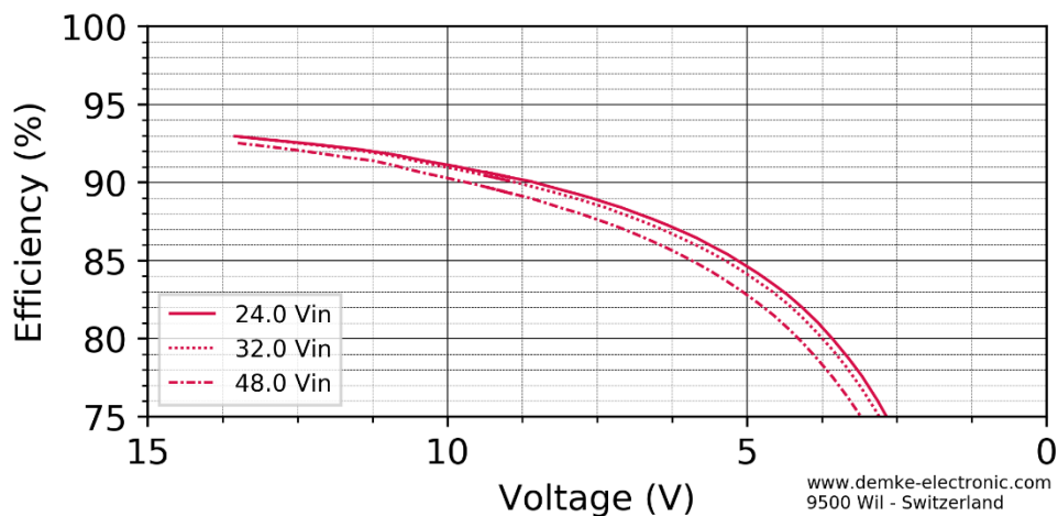
Figure 3 Efficiency in the constant current range of the DC-Transformer 151DH-13.8-On
