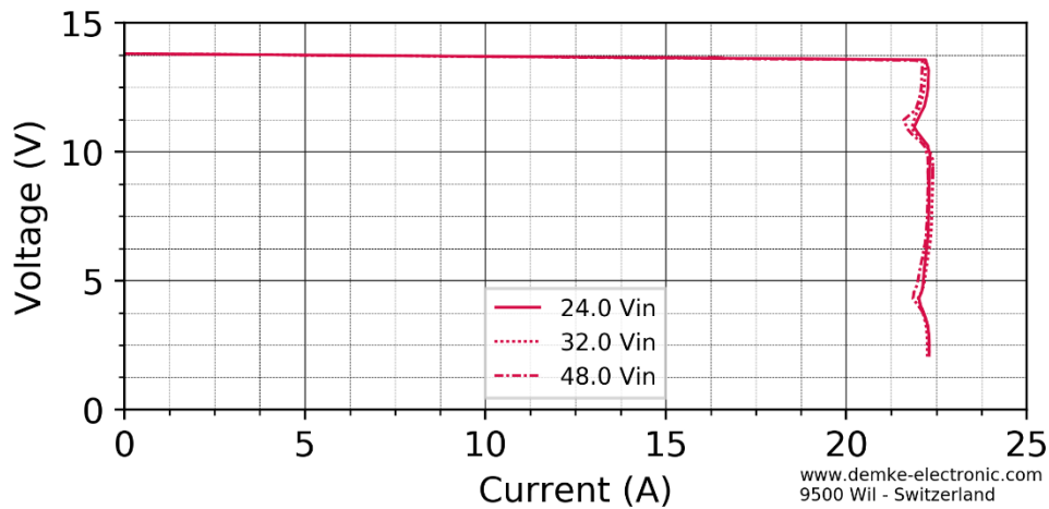
Figure 1 Voltage against current of the DC-Transformer 151DH-13.8-On
