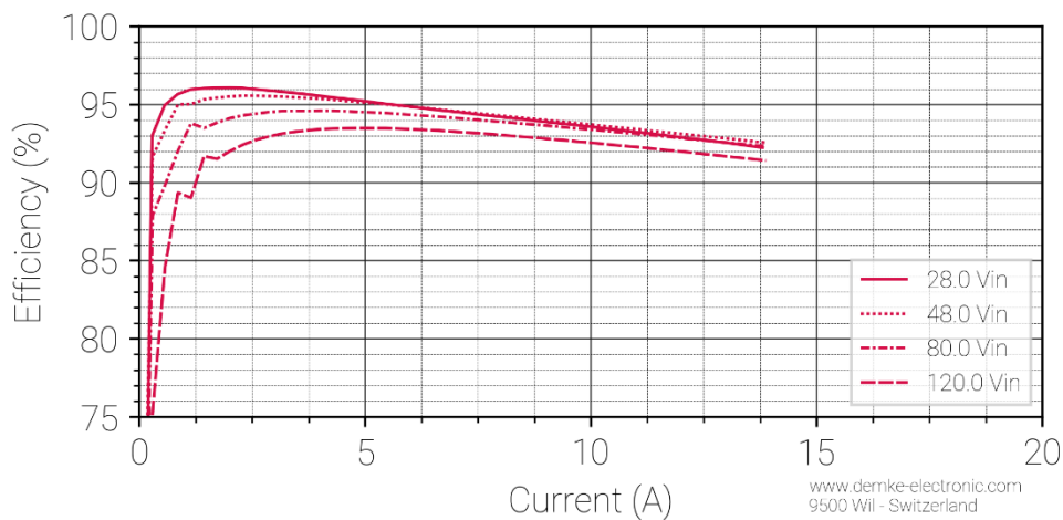
Figure 2 Efficiency in the constant voltage range of the DC-Transformer 154-24
