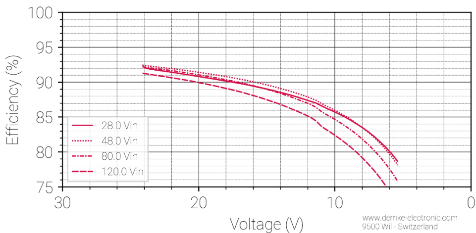
Figure 3 Efficiency in the constant current range of the DC-Transformer 154-24
