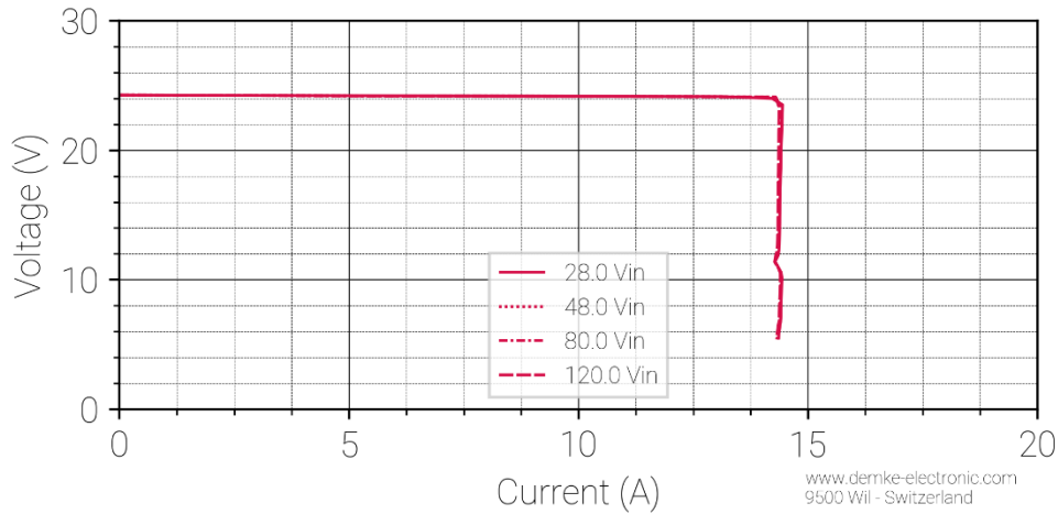
Figure 1 Voltage against current of the DC-Transformer 154-24
