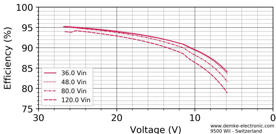
Figure 3 Efficiency in the constant current range of the DC-Transformer 154DH-27-0N
