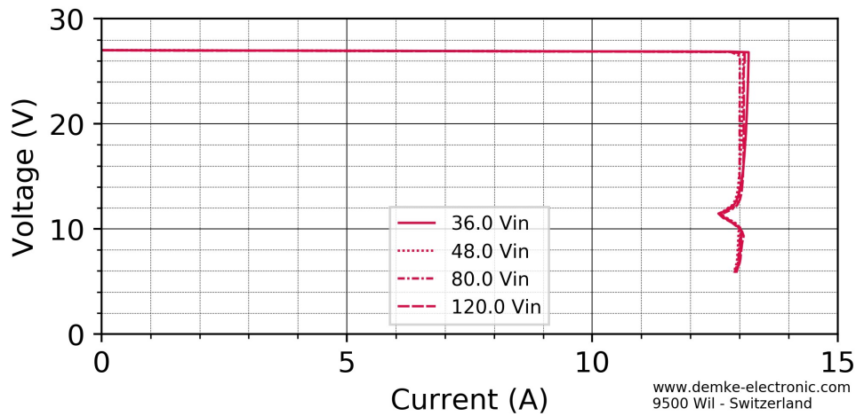
Figure 1 Voltage against current of the DC-Transformer 154DH-27-0N
