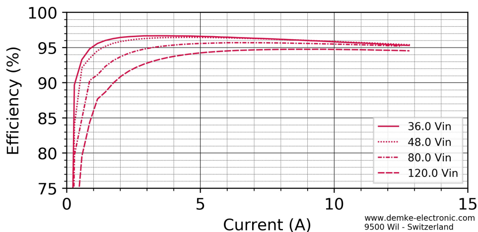
Figure 2 Efficiency in the constant voltage range of the DC-Transformer 154DH-27-0N
