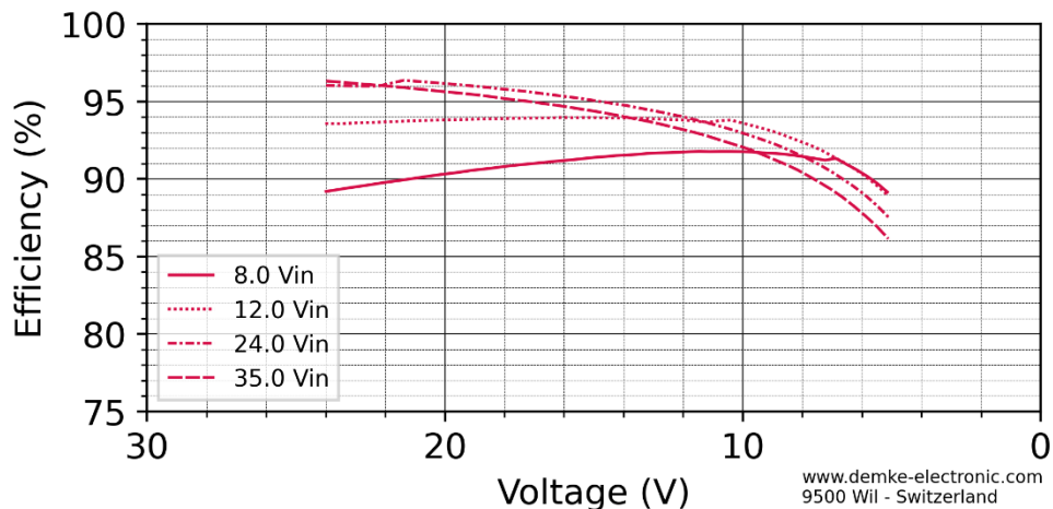
Figure 3 Efficiency in the constant current range of the DC-Transformer 257LEX-24-SD
