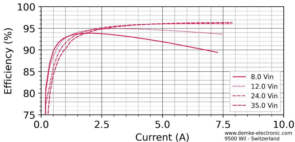
Figure 2 Efficiency in the constant voltage range of the DC-Transformer 257LEX-24-SD
