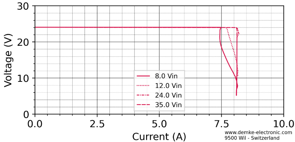
Figure 1 Voltage against current of the DC-Transformer 257LEX-24-SD
