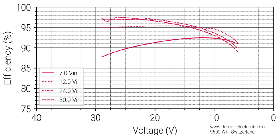
Figure 3 Efficiency in the constant current range of the DC-Transformer 257LE1-29
