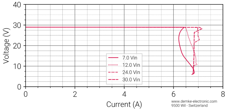
Figure 1 Voltage against current of the DC-Transformer 257LE1-29
