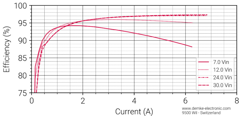
Figure 2 Efficiency in the constant voltage range of the DC-Transformer 257LE1-29
