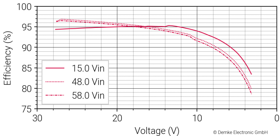
Figure 3 Efficiency in the constant current range of the DC-Transformer 258E1-27.5-ON
