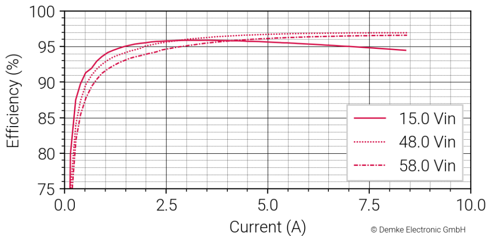
Figure 2 Efficiency in the constant voltage range of the DC-Transformer 258E1-27.5-ON
