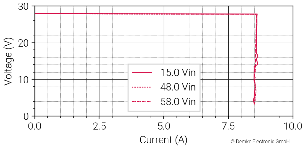
Figure 1 Voltage against current of the DC-Transformer 258E1-27.5-ON
