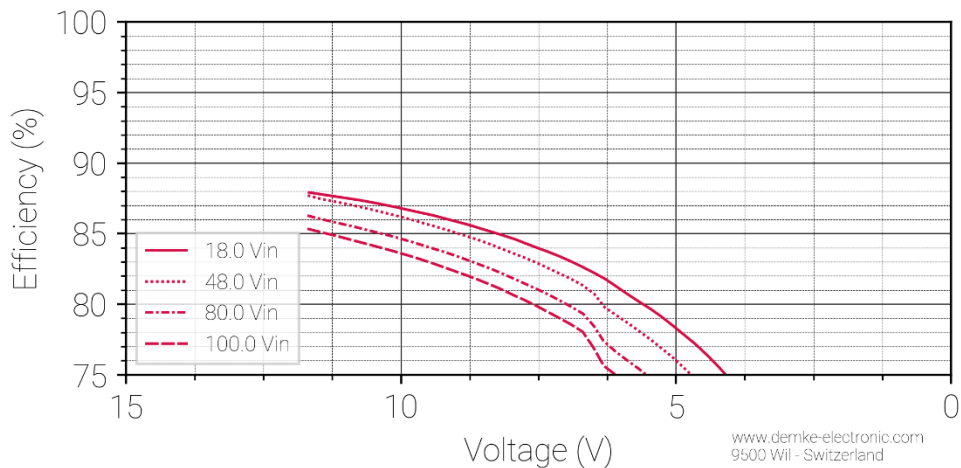
Figure 3 Efficiency in the constant current range of the DC-Transformer 334W-12-SD
