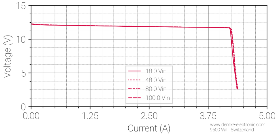
Figure 1 Voltage against current of the DC-Transformer 334W-12-SD
