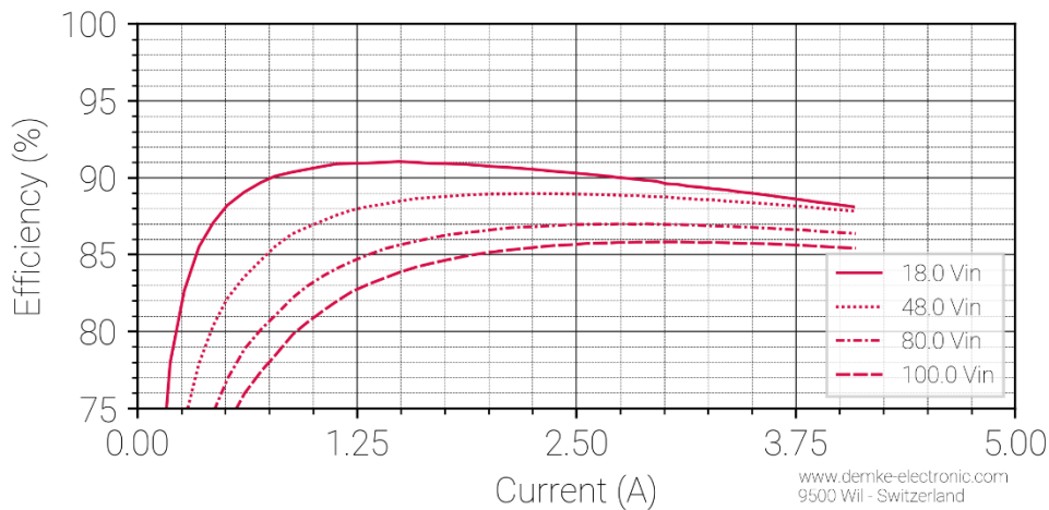
Figure 2 Efficiency in the constant voltage range of the DC-Transformer 334W-12-SD
