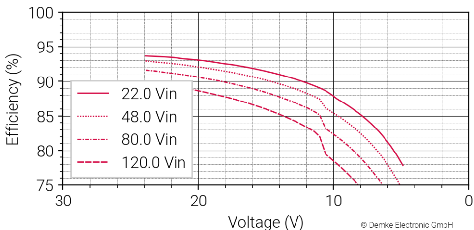
Figure 3 Efficiency in the constant current range of the DC-Transformer 344-24
