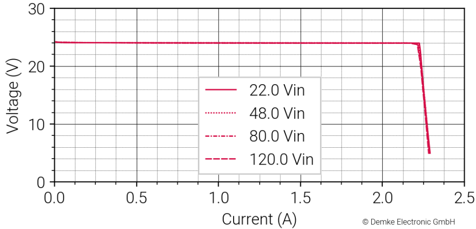
Figure 1 Voltage against current of the DC-Transformer 344-24
