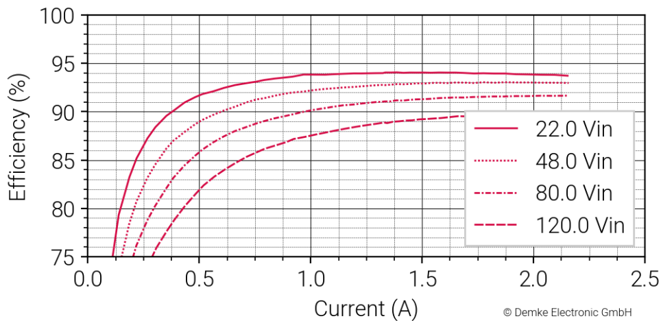
Figure 2 Efficiency in the constant voltage range of the DC-Transformer 344-24
