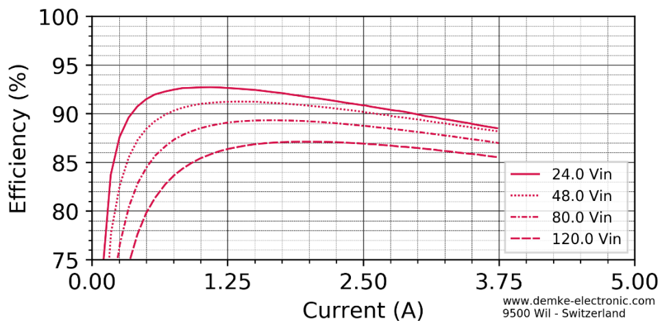
Figure 2 Efficiency in the constant voltage range of the DC-Transformer 354W1-24024-SD single output
