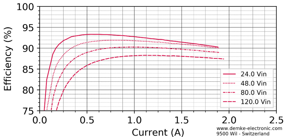
Figure 5 Efficiency in the constant voltage range of the DC-Transformer 354W1-24024-SD bipolar output
