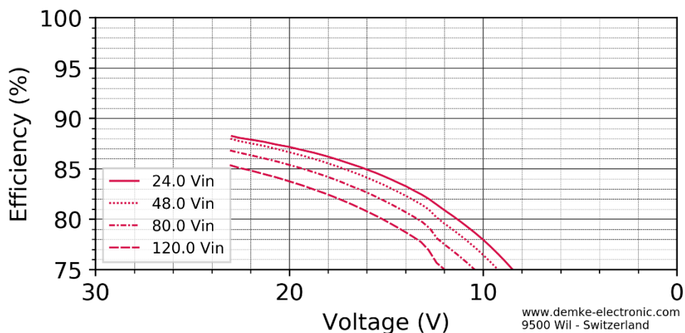
Figure 3 Efficiency in the constant current range of the DC-Transformer 354W1-24024-SD single output
