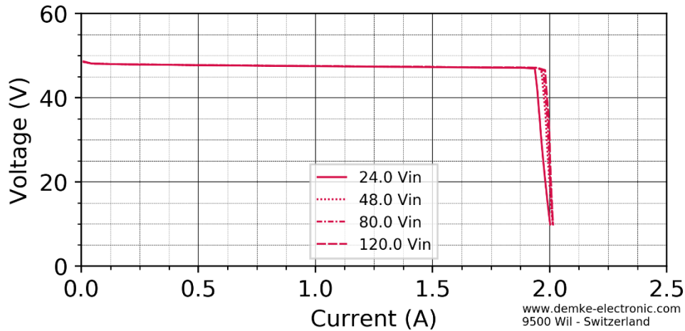
Figure 4 Voltage against current of the DC-Transformer 354W1-24024-SD bipolar output
