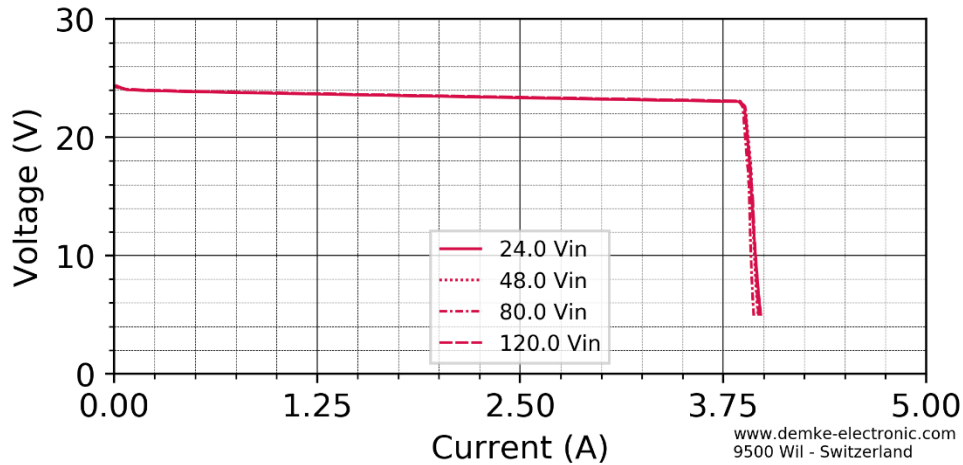
Figure 1 Voltage against current of the DC-Transformer 354W1-24024-SD single output
