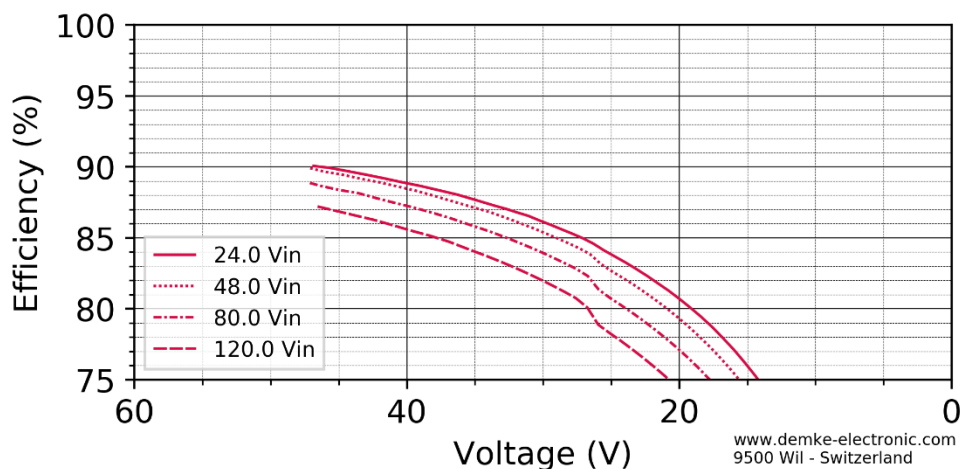
Figure 6 Efficiency in the constant current range of the DC-Transformer 354W1-24024-SD bipolar output
