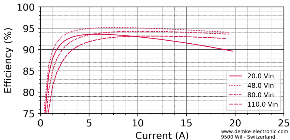
Figure 2 Efficiency in the constant voltage range of the DC-Transformer 755-24-SD
